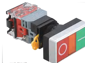
双位带灯钮 Double head Illuminated momentary push button LA36- \odot D / \triangle
