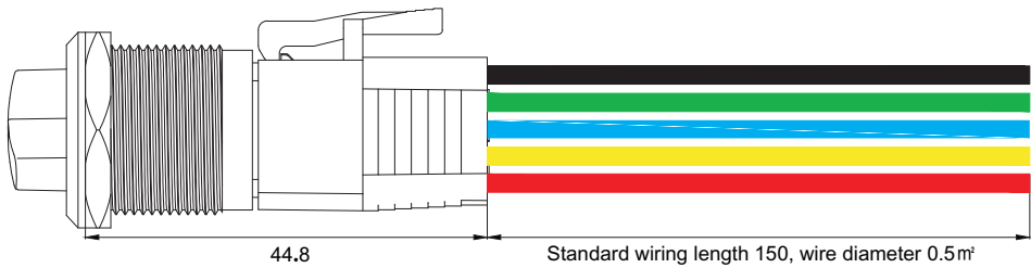
Combination diagram of selector switch and socket
