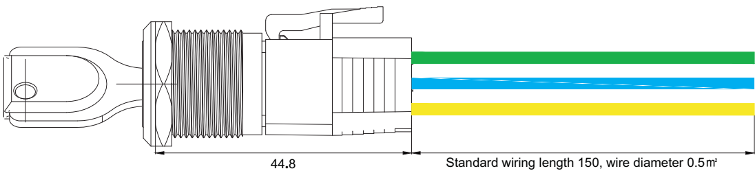
Combination diagram of key-lock selector switch and socket
