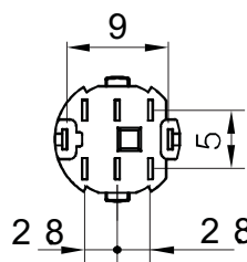
2NO2NC, Terminal(1.8×0.4)
