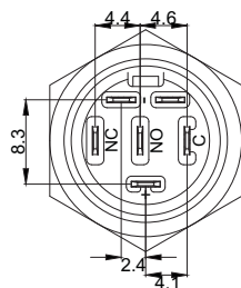
1NO1NC, Terminal(2.8×0.5)
