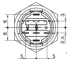
Bottom view of emergency, selector and key-lock selector switch
