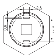
Pin terminal
